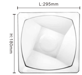
LARGE FRUIT PLATE No. PL-B712QUA/BHA1 D:295 H:18 SPF:1PC/SET,6SETS/CTN CBM:0.021 G.W.:13.0KG
